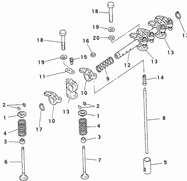
FIG.127 TIMING PARTS
