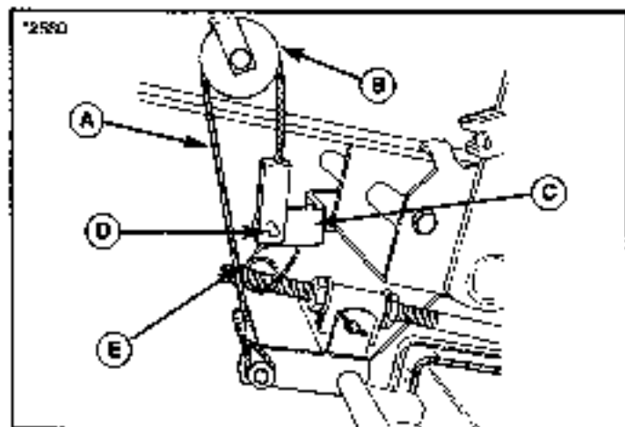
Figure 7. Mower With Manual Lift (Left Side Shown)
