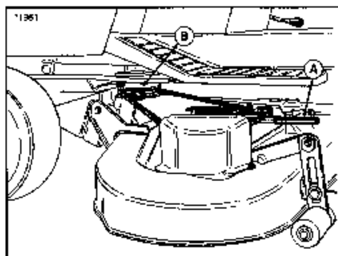
Figure 9. Installing Belt
