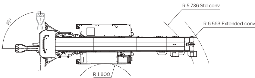
Turning radius
