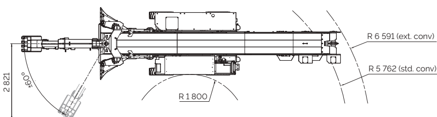
Turning radius
