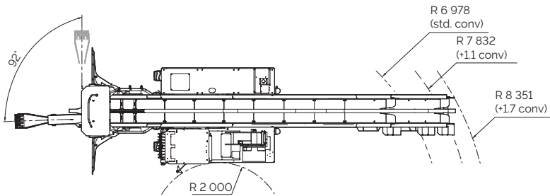
Turning radius
