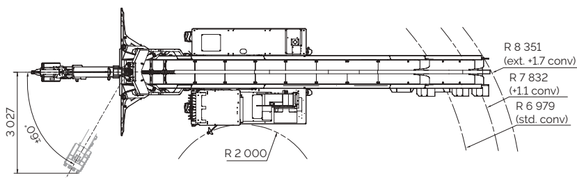
Turning radius
