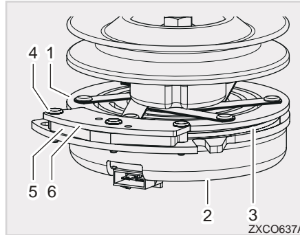
(1) Armature (4) Brake Mounting Bolt (2) Field Shell (5) Brake Spacer (3) Rotor (6) Brake Pole
