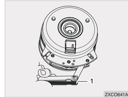
(1) Feeler Gauge
