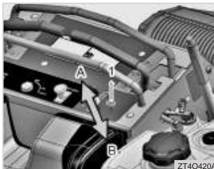
(1) Choke Lever (A) ON (B) OFF
