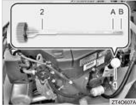
(1) Oil Filler Neck (2) Oil Dipstick (A) Upper Limit (B) Lower Limit
