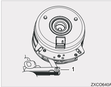
(1) Feeler Gauge
