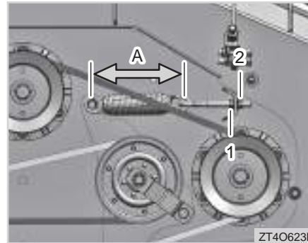
(1) Nut 1 (2) Nut 2 (A) Adjusting Length of Belt Tension
