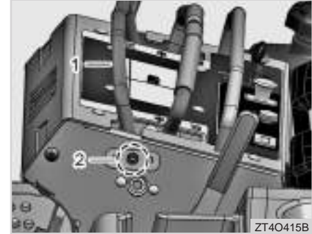
(1) Reference Control Front Lever (2) Adjust Bolt
