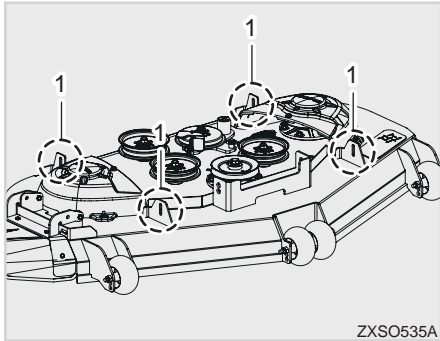
(1) Lifting Position
