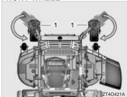
(1) Wheel &amp; Wheel Support Fork Bracket
