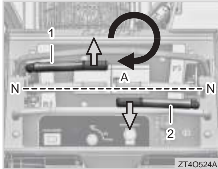
(1) LH Steering Levers (2) RH Steering Levers (A) Right Zero Turn
