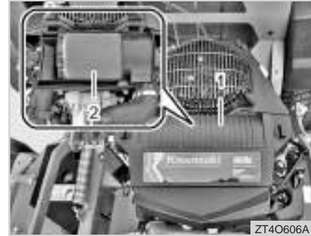
(1) Air Cleaner Cover (2) Locking Cap (3) Air Cleaner Element
