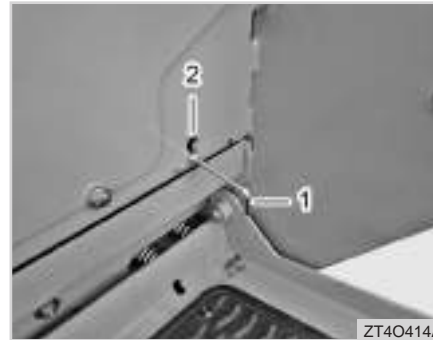
(1) Bypass Control Rod (2) Opening
