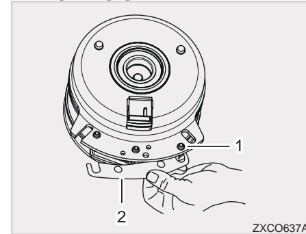
(1) Brake Mounting Bolt (2) Shim
