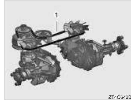
(1) Drive Belt
