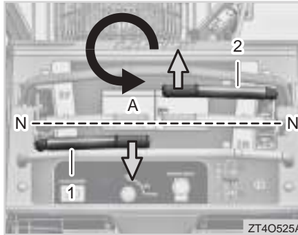
(1) LH Steering Levers (2) RH Steering Levers (A) Left Zero Turn
