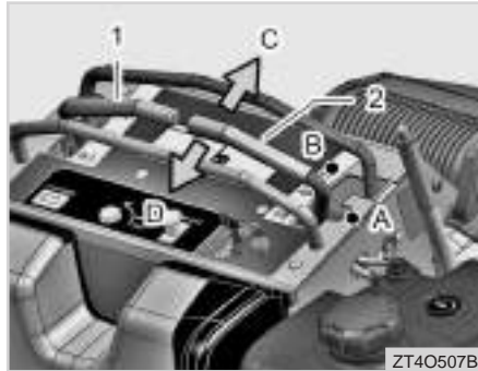
(1) LH Steering Levers (2) RH Steering Levers (A) Neutral Lock (B) Forward (C) Neutral (D) Reverse
